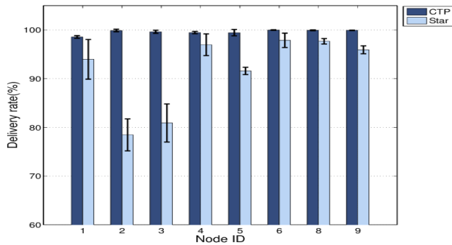
4. CTP delivery rate vs. the star protocol under static conditions for 8 nodes network. CTP achieves reliable performance across all nodes.
